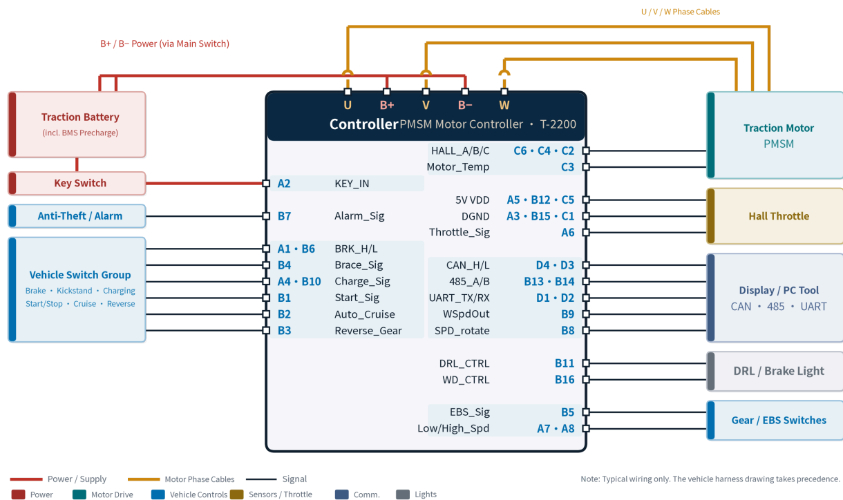
Figure 10-1 T-2200 Typical Vehicle Wiring Diagram
