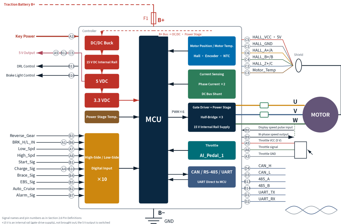
Figure 5-1 T-2200 System Block Diagram
