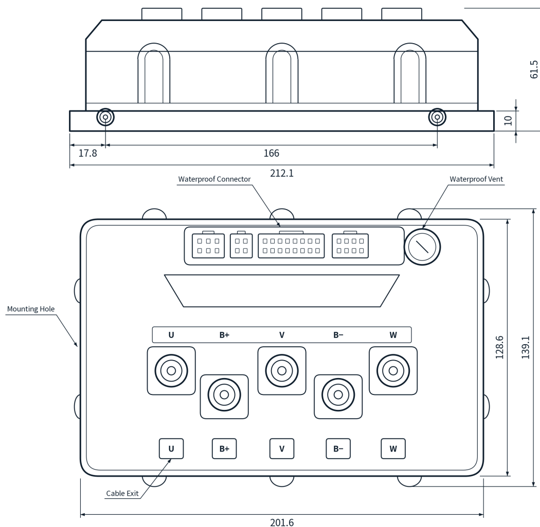
Figure 7-1 Outline and Interface Dimensions (mm)
