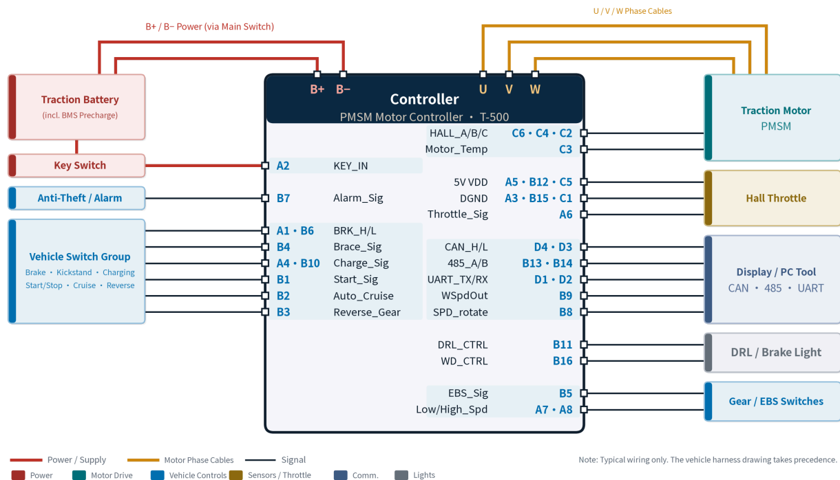
Figure 10-1 T-500 Typical Vehicle Wiring Diagram
