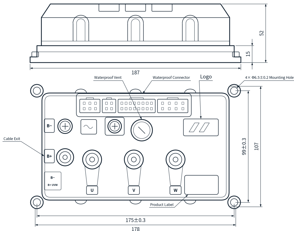
Figure 7-1 Outline and Interface Dimensions (mm)
