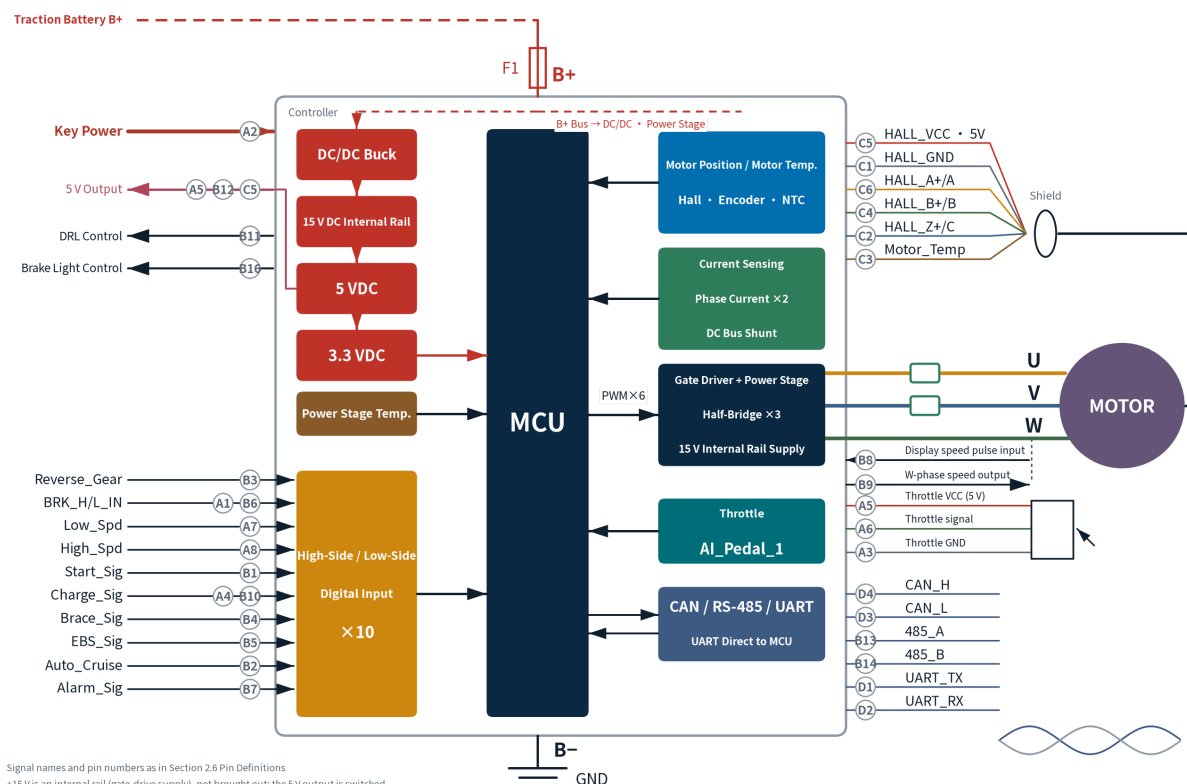
Figure 5-1 T-500 System Block Diagram
